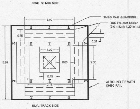
PLAN OF PROPOSED RAIL GUARDING AROUND SPRINKLER STRUCTURE
