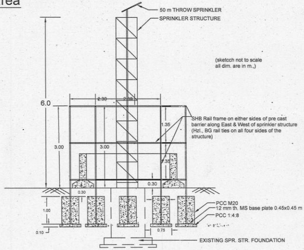
SECTIONAL ELEVATION OF PROPOSED RAIL GUARDING AROUND SPRINKLER STRUCTURE
